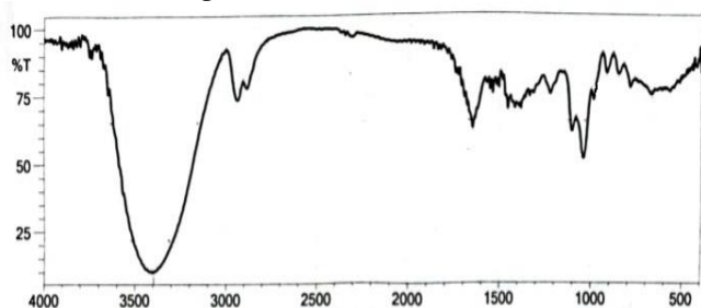
Figure 4. FTIR for control sample
